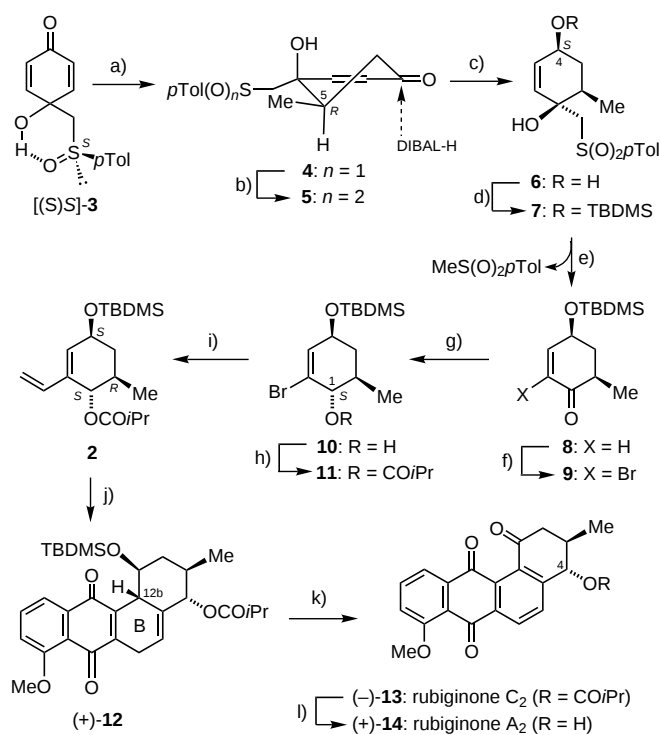
Scheme 2. Enantioselective total synthesis of rubiginones \text{A}_2 and \text{C}_2 : a) \text{AlMe}_3 , \text{CH}_2\text{Cl}_2 , -78^\circ\text{C} , 4 h, 65%; b) MCPBA, \text{CH}_2\text{Cl}_2 , 0^\circ\text{C} , 30 min, 96%; c) DIBAL-H, THF, -78^\circ\text{C} , 30 min, 99%; d) TBDMSOTf, 2,6-lutidine, \text{CH}_2\text{Cl}_2 , 0^\circ\text{C} , 2 h; e) \text{Cs}_2\text{CO}_3 , \text{CH}_3\text{CN} , room temperature, 17 h, 87% over two steps; f) \text{Br}_2 , \text{CCl}_4 , 0^\circ\text{C} , then \text{Et}_3\text{N} , room temperature, 32 h, 80%; g) \text{LiAlH}_4 , THF, -100^\circ\text{C} , 30 min; h) i\text{PrCOCl} , DMAP, \text{CH}_2\text{Cl}_2 , 1 h, 79% over two steps; i) [\text{Pd}(\text{PPh}_3)_4] , [\text{CH}_2=\text{CHSnBu}_3] , toluene, 90^\circ\text{C} , 24 h, 78%; j) (\pm)\text{-1} (2 equiv), \text{CH}_2\text{Cl}_2 , reflux, 24 h, 52%; k) h\nu , air, room temperature, 16 h, 35%; l) \text{K}_2\text{CO}_3 , THF/MeOH, room temperature, 90 min, 91%. MCPBA = meta -chloroperbenzoic acid; DIBAL-H = diisobutylaluminum hydride; TBDMSOTf = tert -butyldimethylsilyl trifluoromethanesulfonate; DMAP = 4-dimethylaminopyridine.
